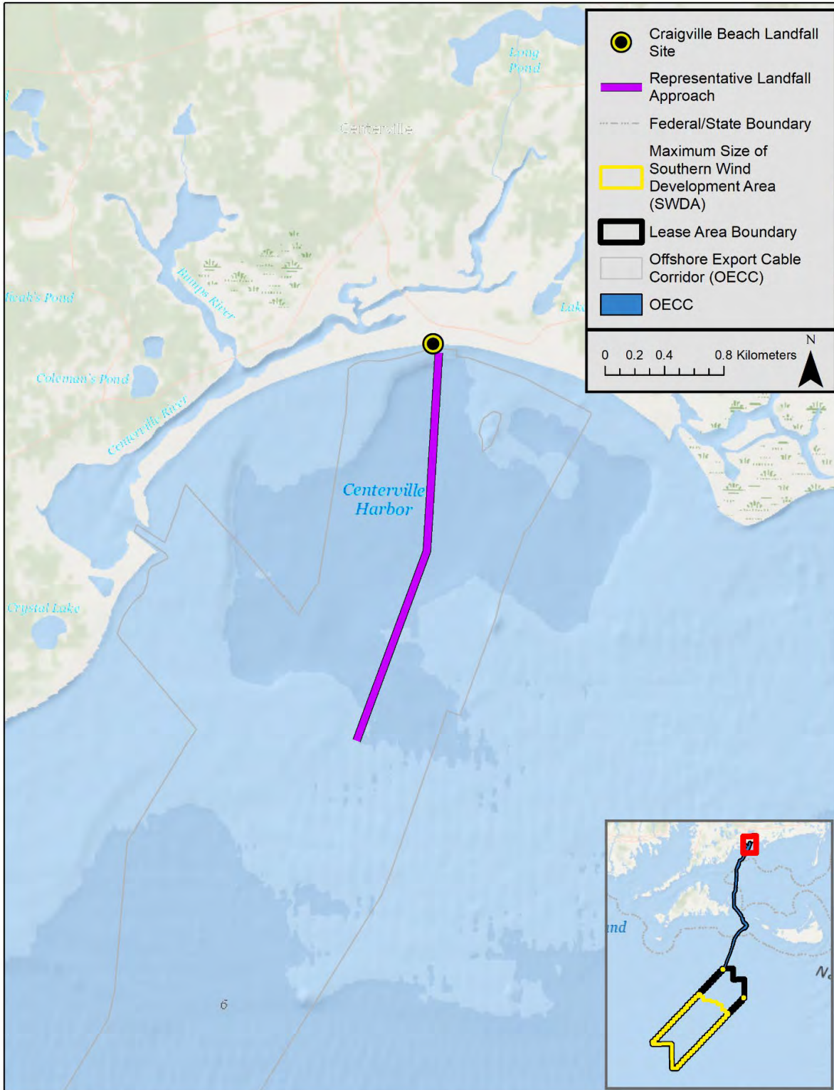
Figure 18. Representative OECC Landfall Approach Route
