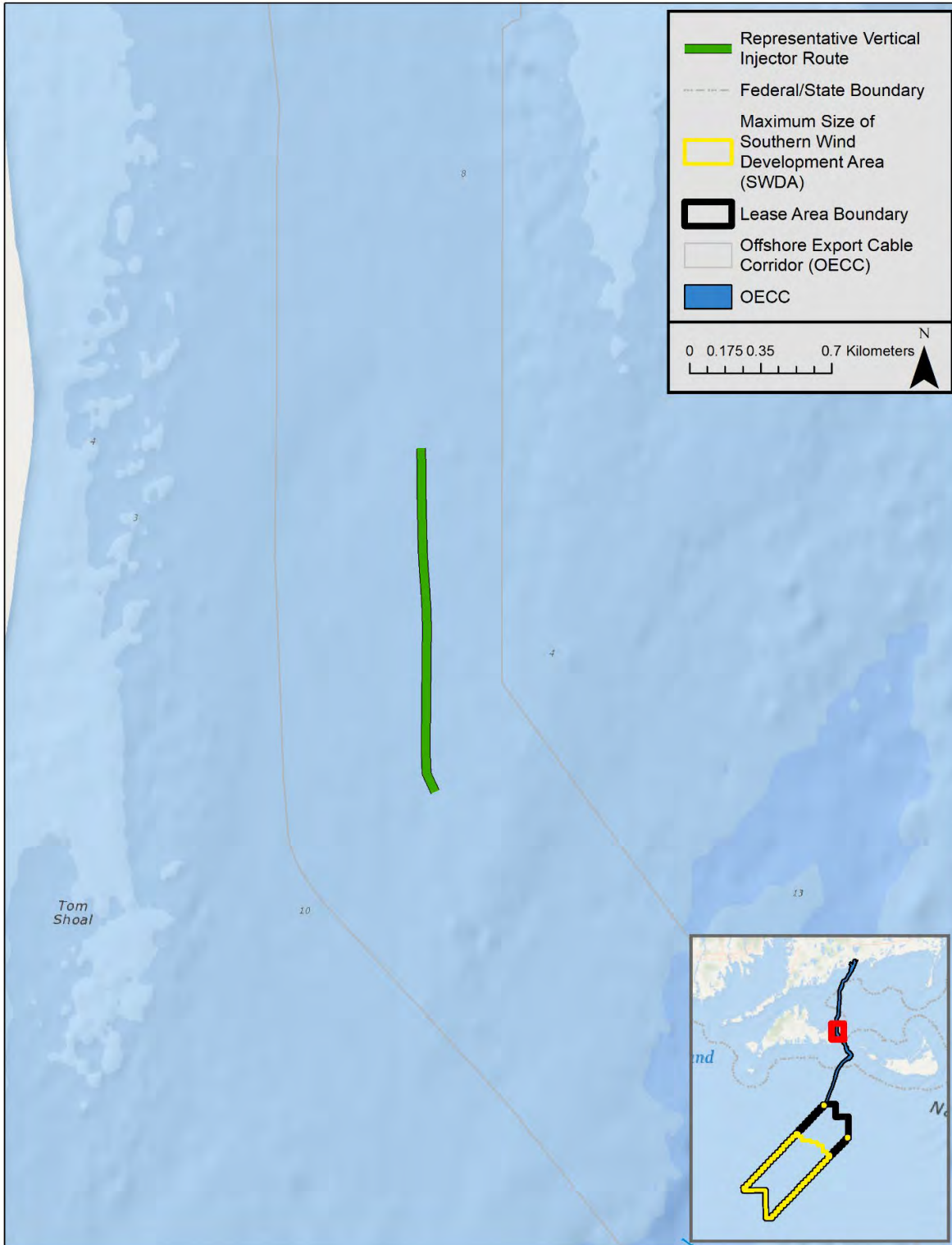
Figure 17. Representative OECC Vertical Injector Route
